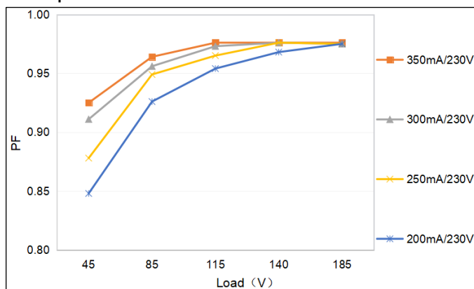
Mains power factor λ
